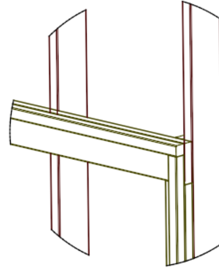
DETAIL A SCALE 1:12
